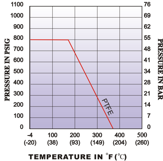
Pressure Vs. Temperature Chart for Valve 1/4" (DN8) to 3" (DN80)
