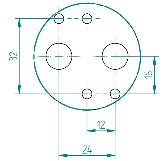
DETAIL A 1:1 NAMUR SOLENOID MOUNTING
